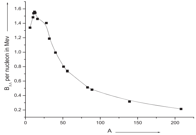
Figure 5. ( B_{\Lambda\Lambda} ) per nucleon versus mass no. (A) for the ground states of double \Lambda -hypernuclei.
